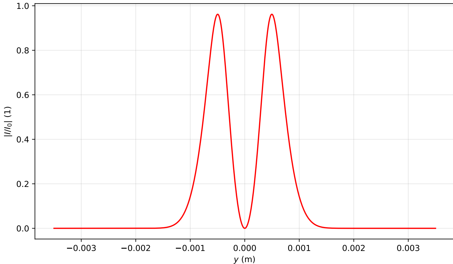
Intensity profile I(x=0, y, z=0.239)/I_0 , P_{in}=5.0P_{cr} , artificial time
